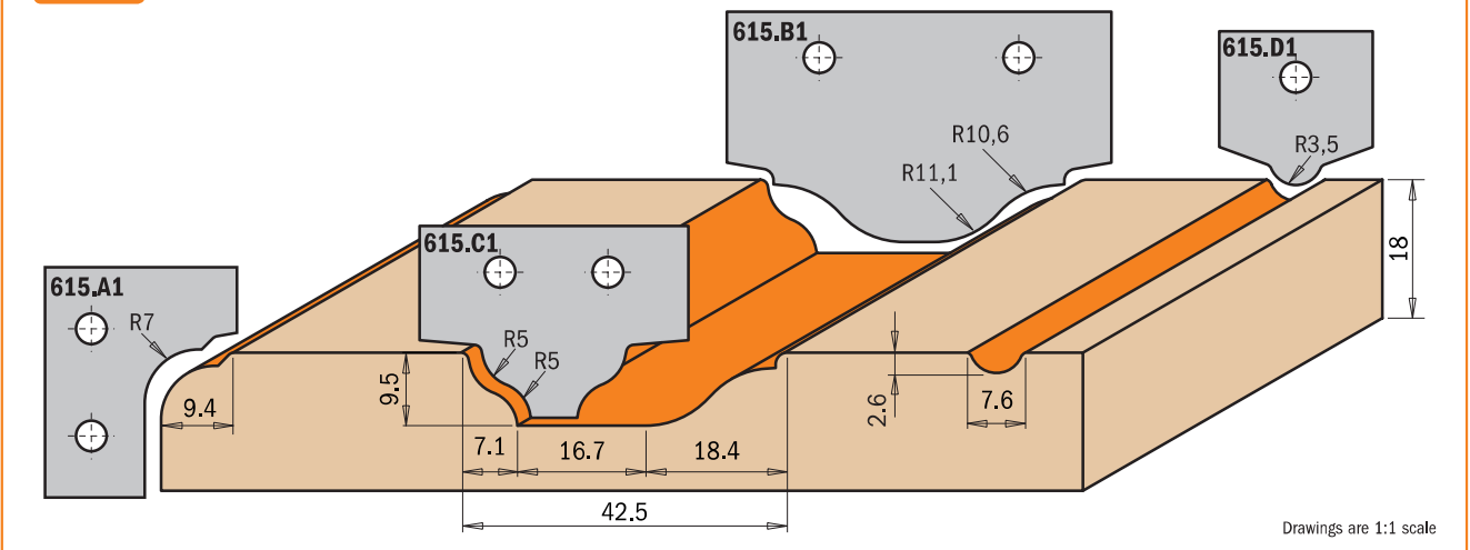
Standard Profile No. 1
