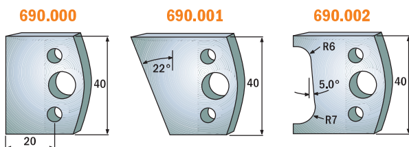
Profile knives cutting length=40mm (serie 690)
